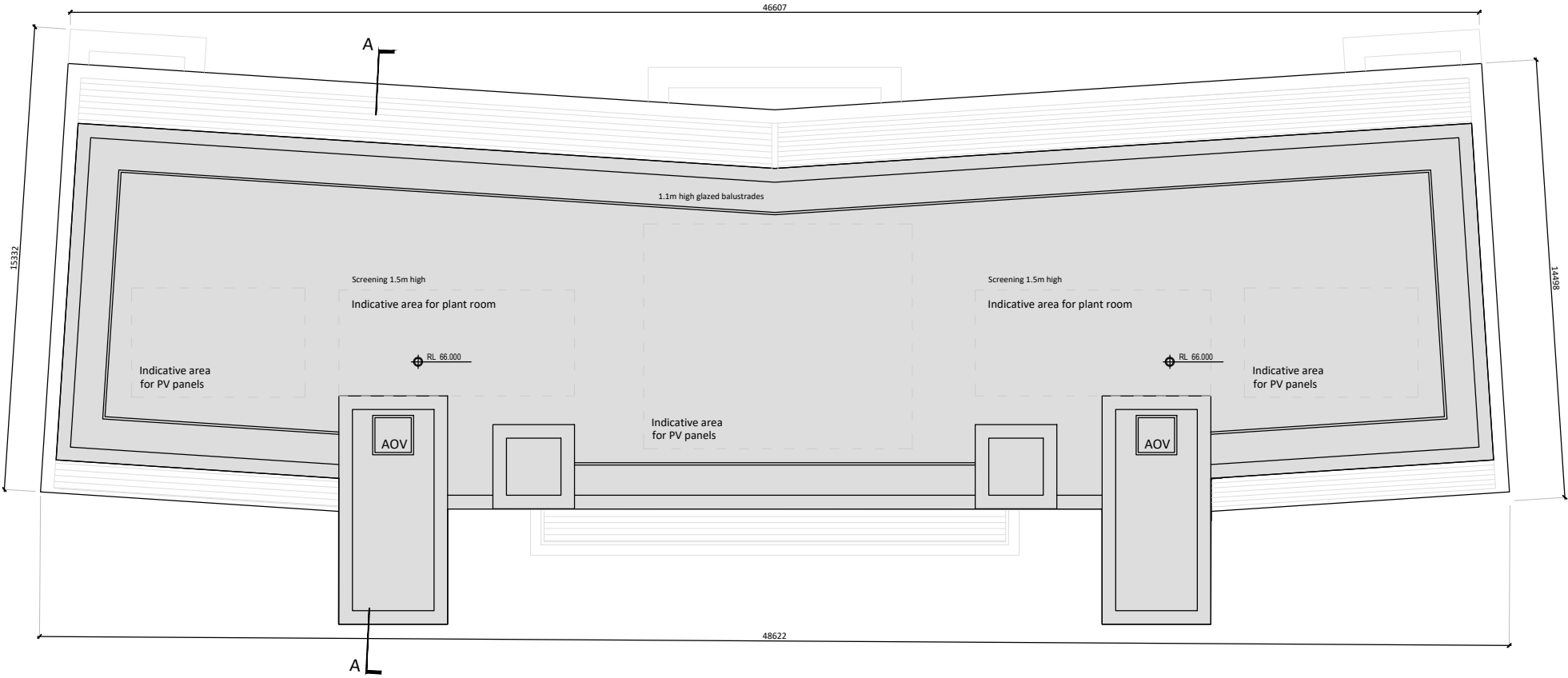
01 Block A - Roof Plan
