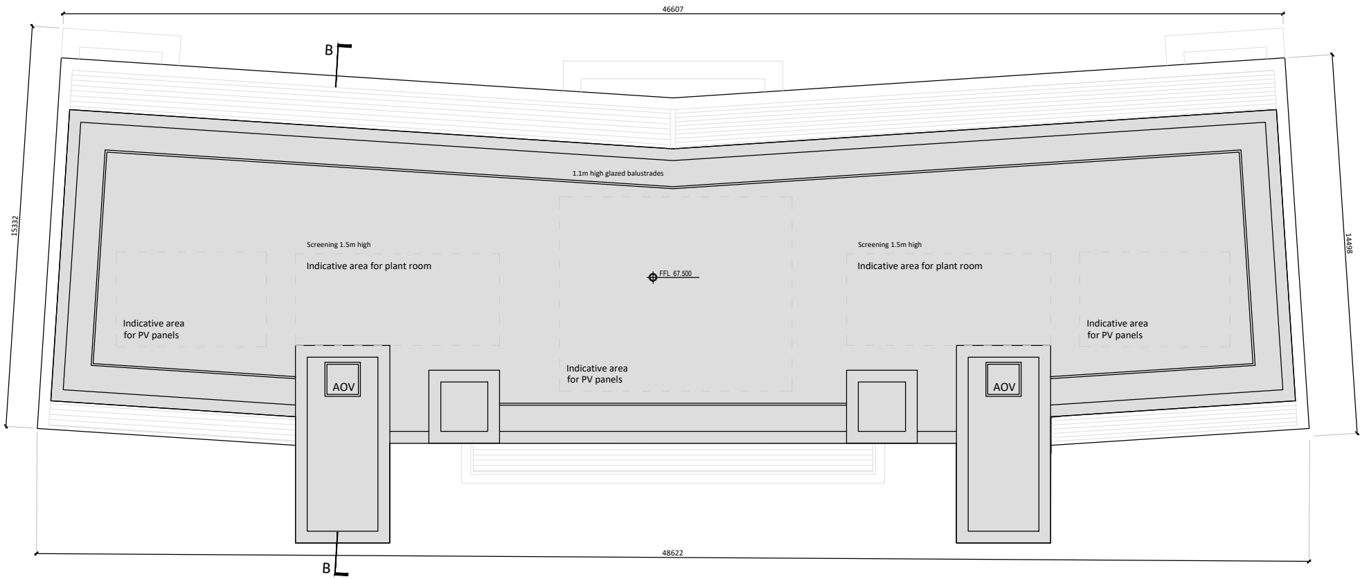
Block B - Roof Plan
