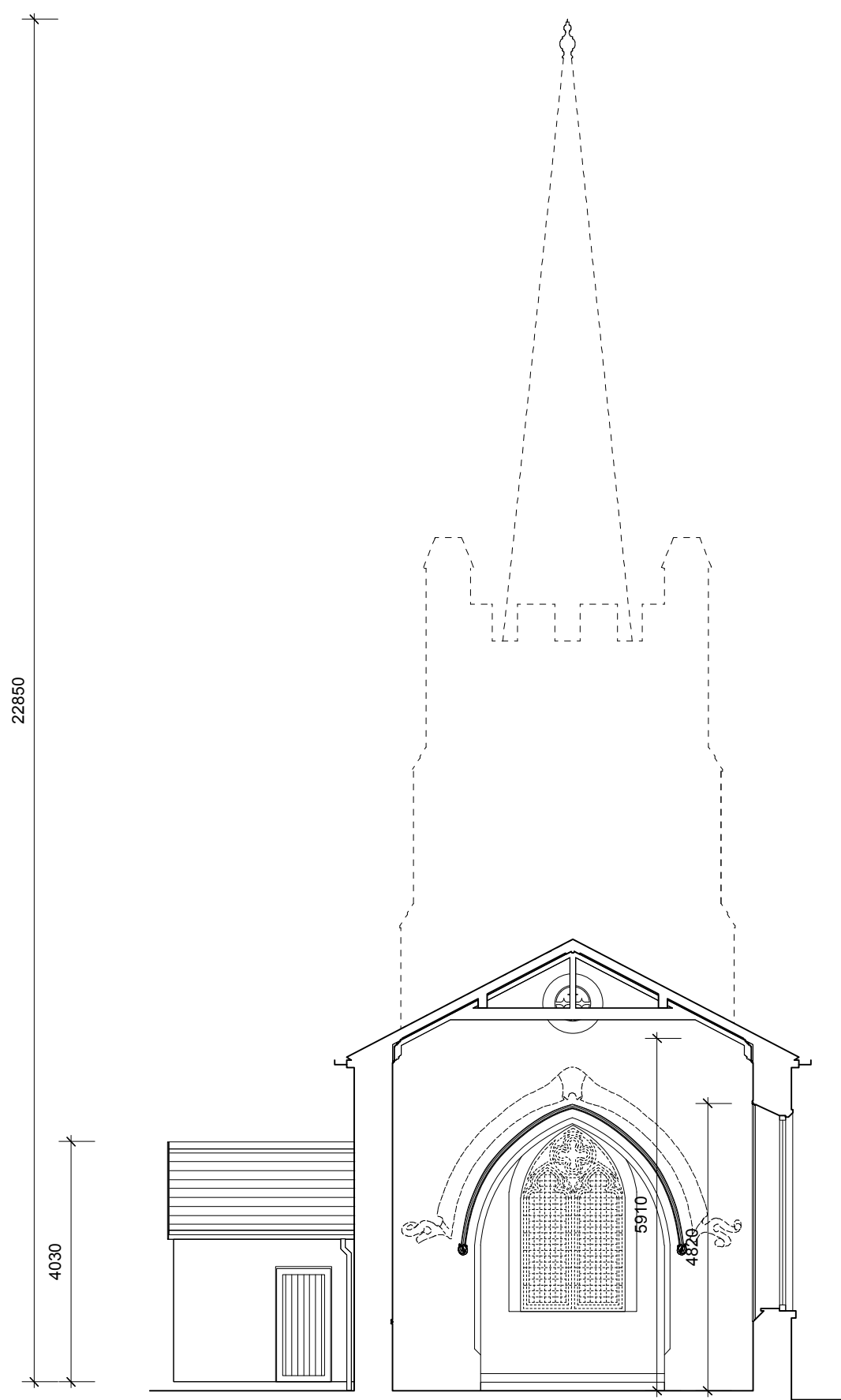
SECTION B-B
