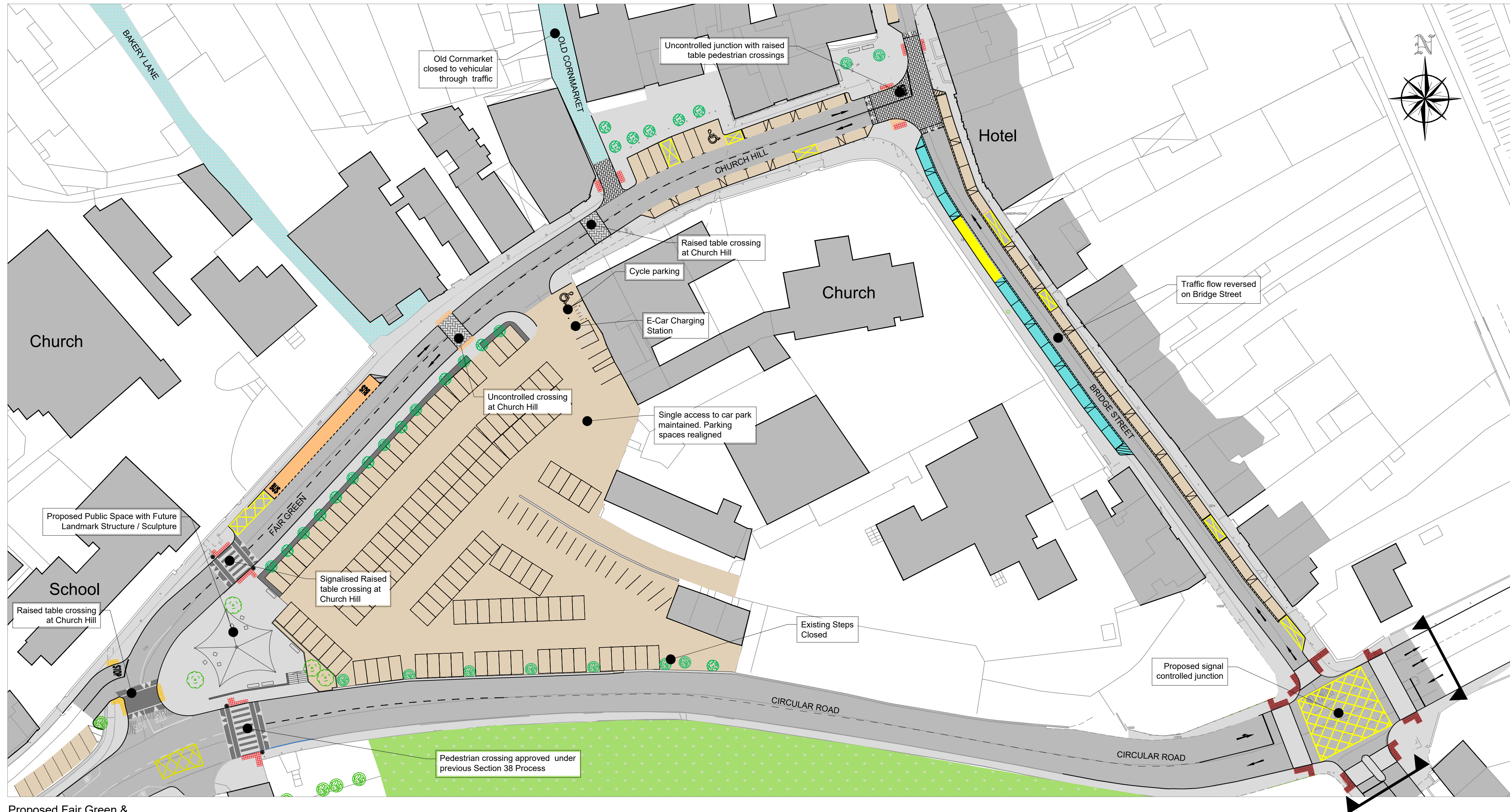
Proposed Fair Green & Church Hill Scale 1:500
