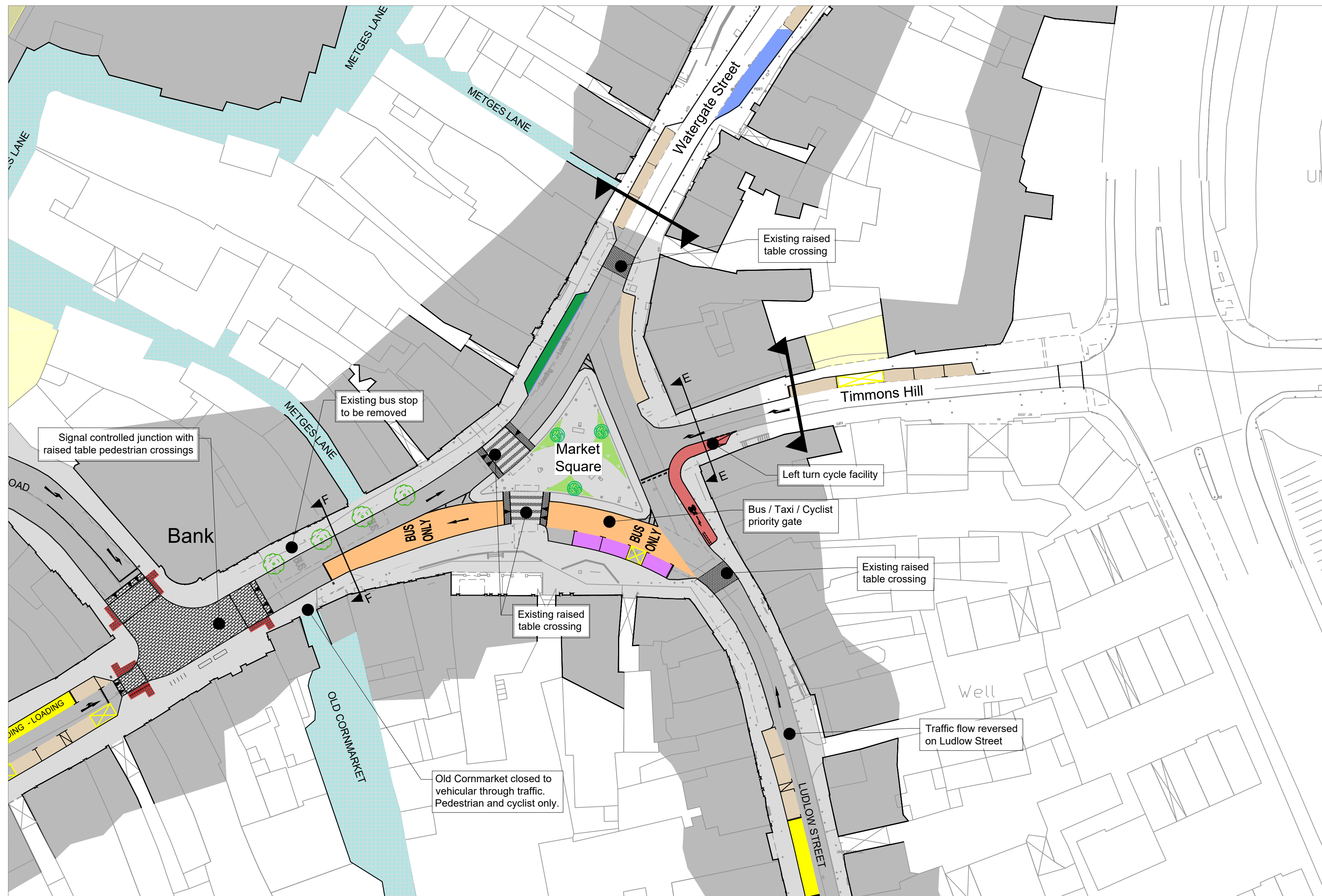
Proposed Market Square Scale 1:500
