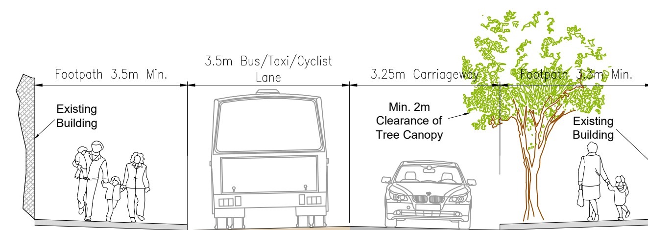
Proposed Section F-F Scale - NTS
