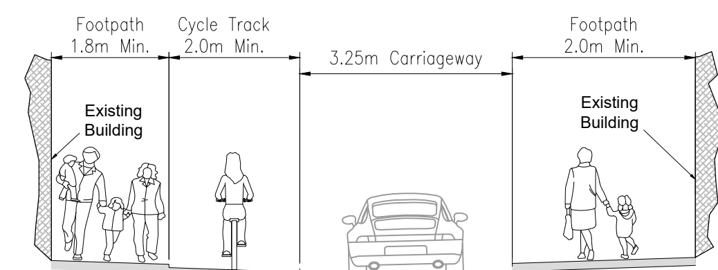
Proposed Section E-E Scale - NTS
