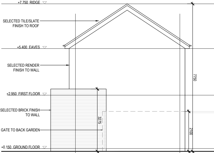
05 H3A - Side Elevation
