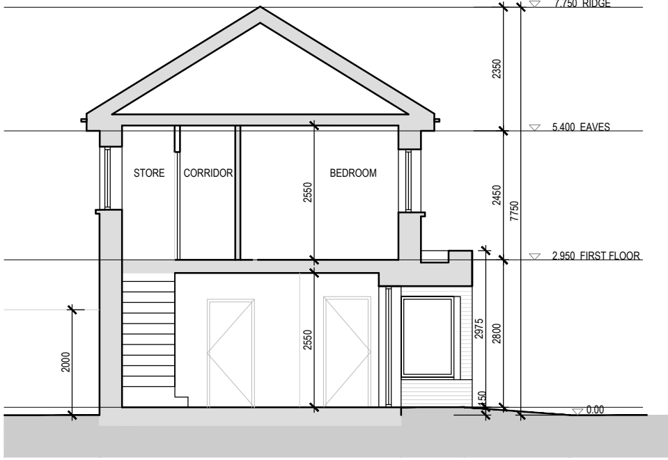
06 H3A - Section AA
