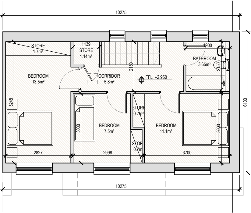
02 H3A -First Floor Plan
