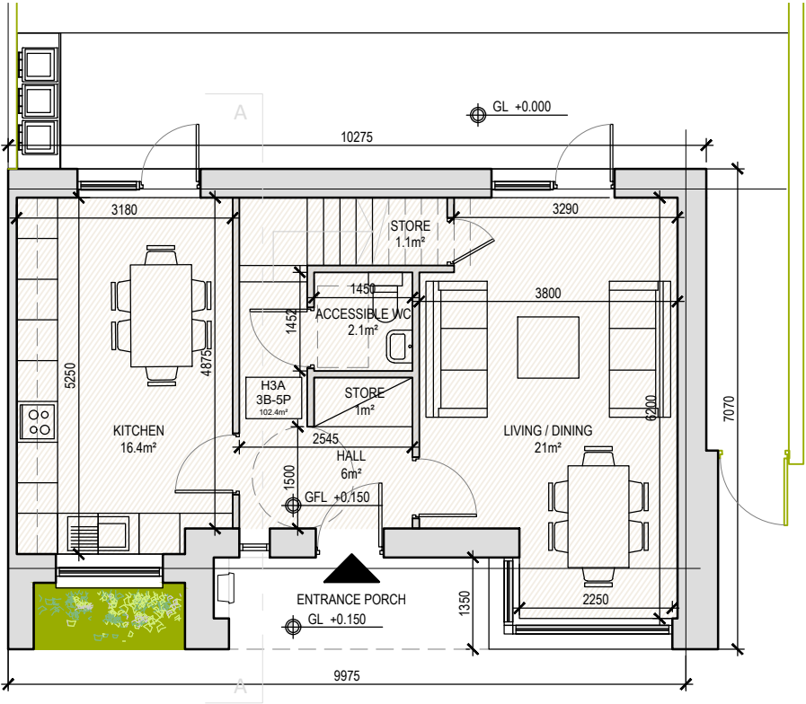
01 H3A - Ground Floor Plan
