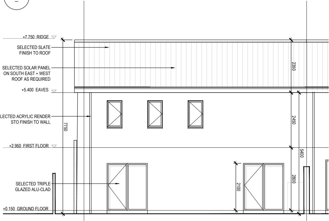
03 H3A - Front Elevation
