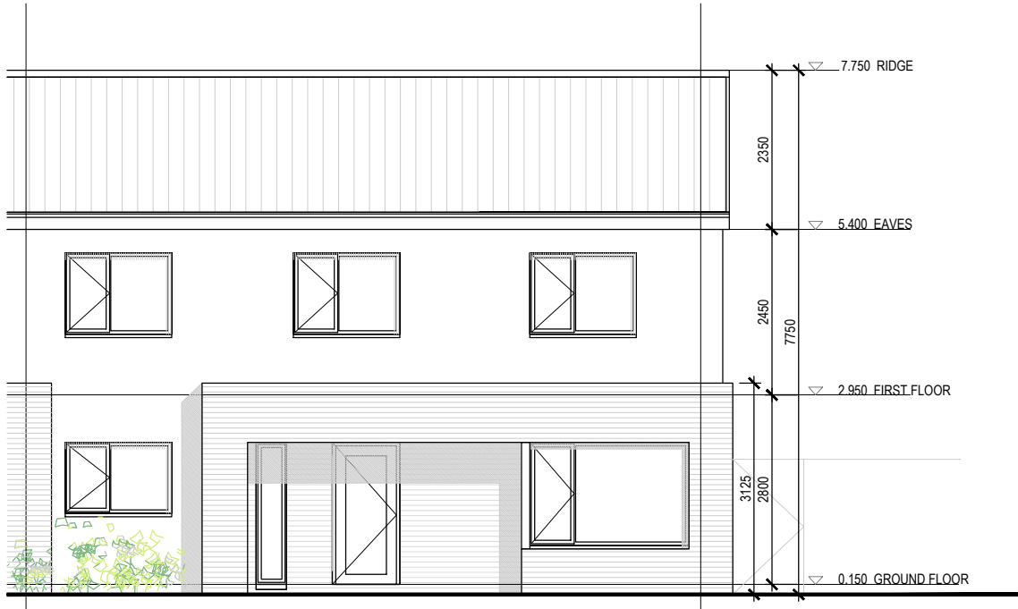
03 H3A - Front Elevation
