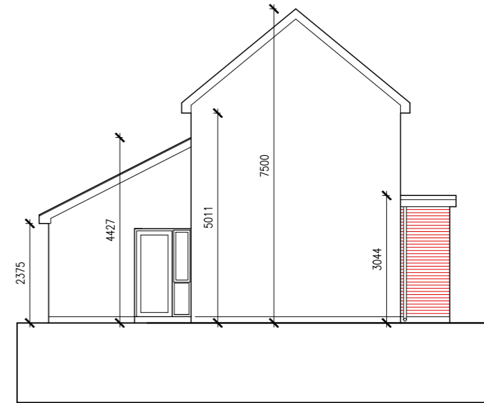
WEST ELEVATION
