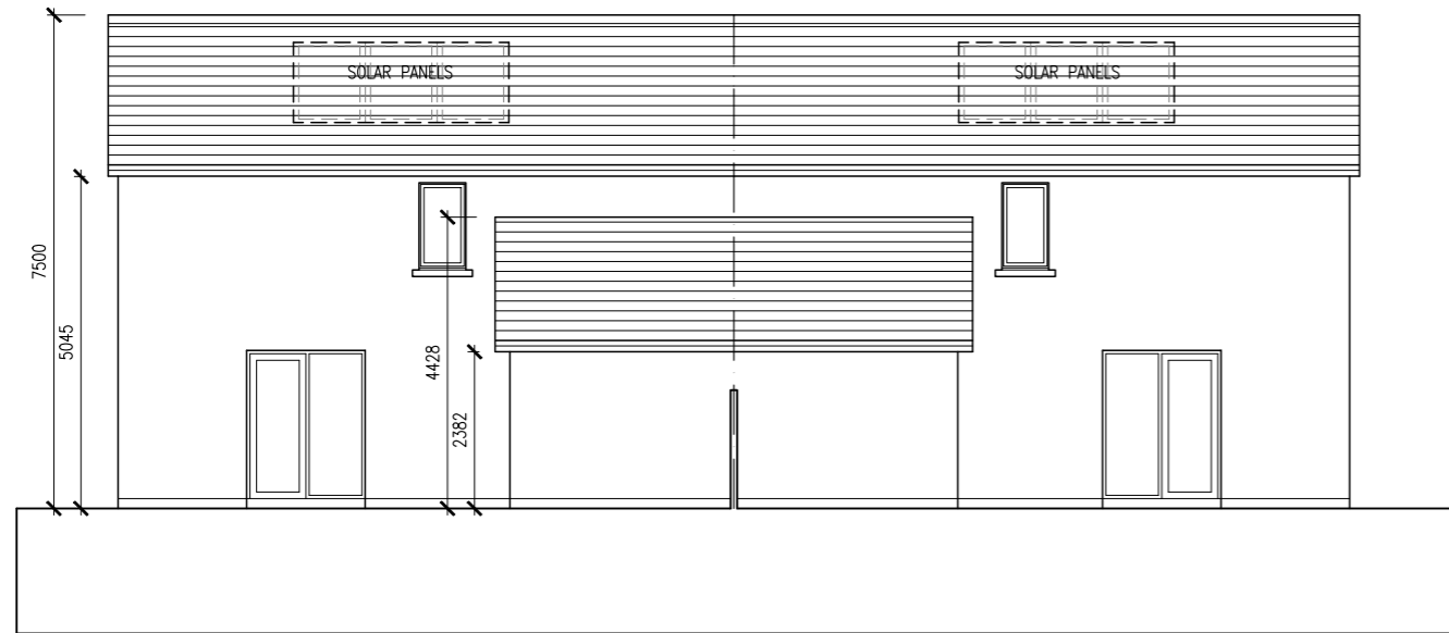
NORTH ELEVATION
