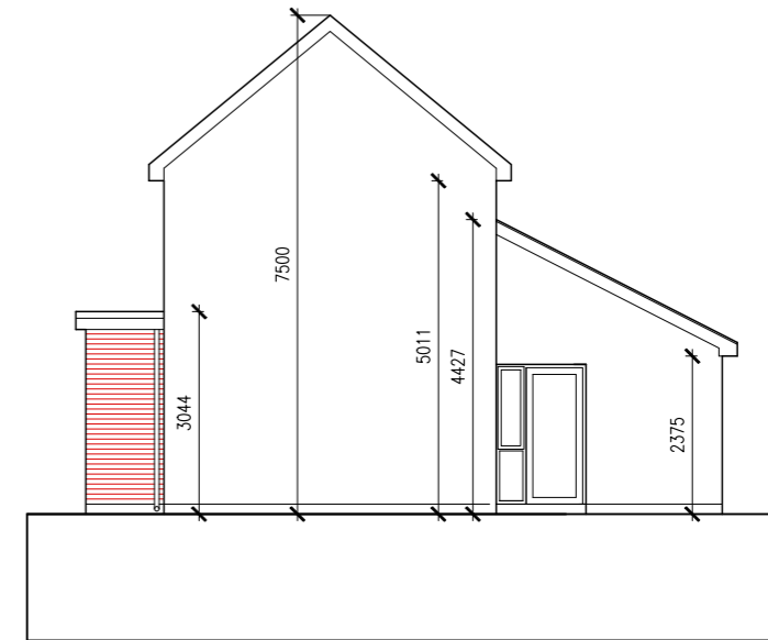
EAST ELEVATION
