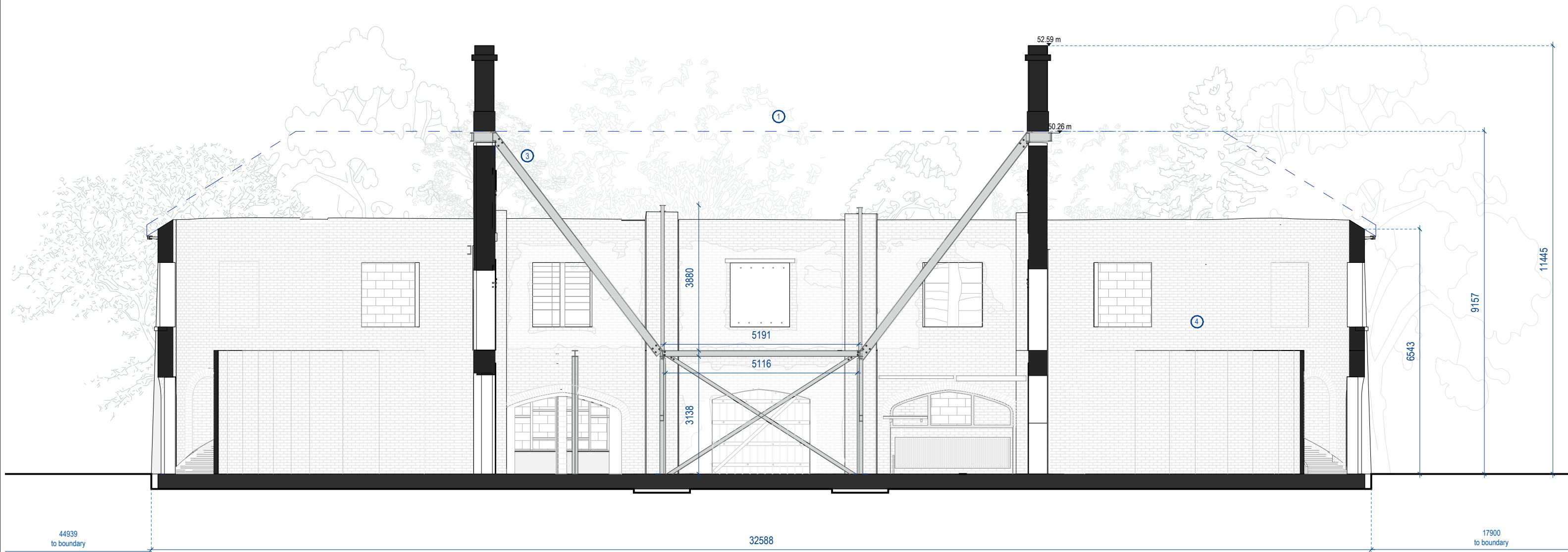
EXISTING BUILDING WITH TEMPORARY STRUCTURAL WORKS
