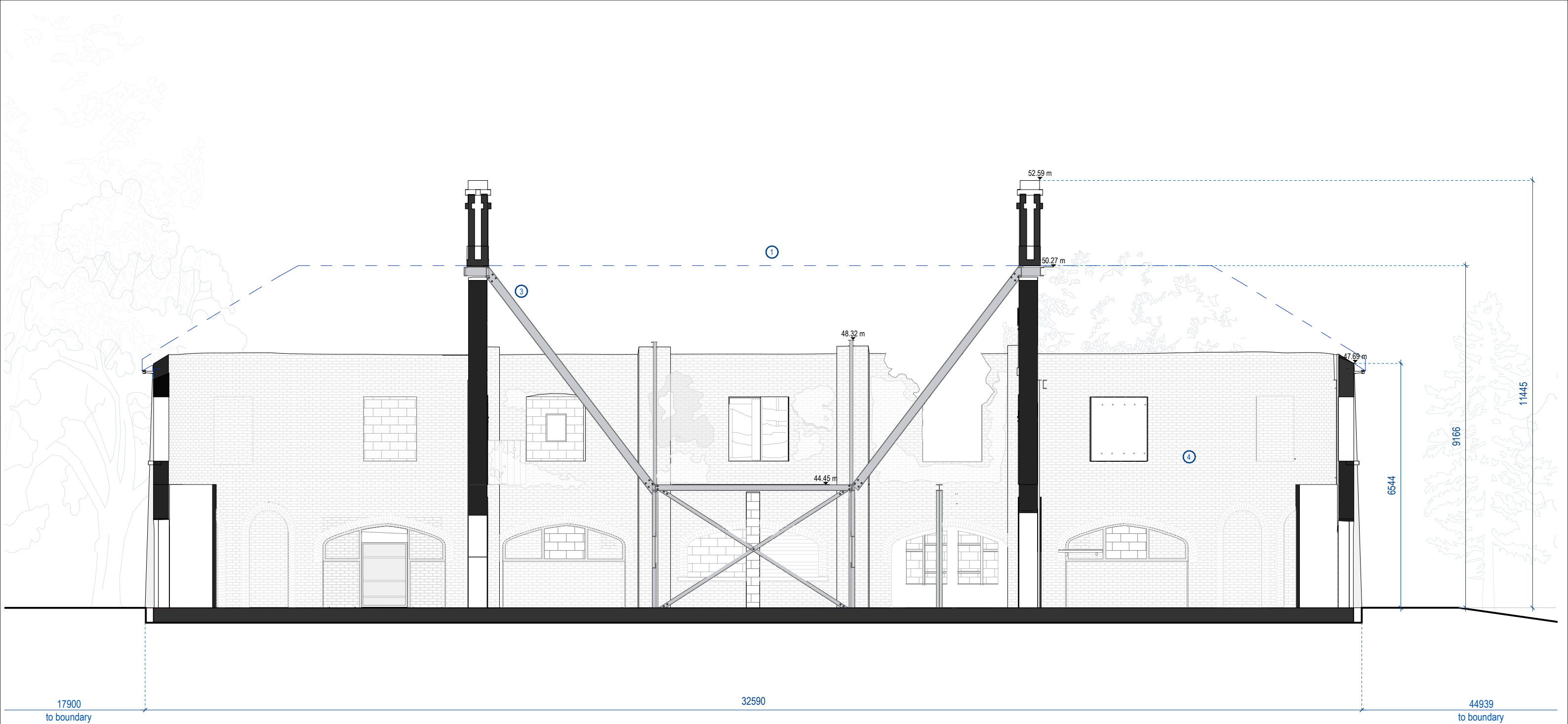
EXISTING BUILDING WITH TEMPORARY STRUCTURAL WORKS
