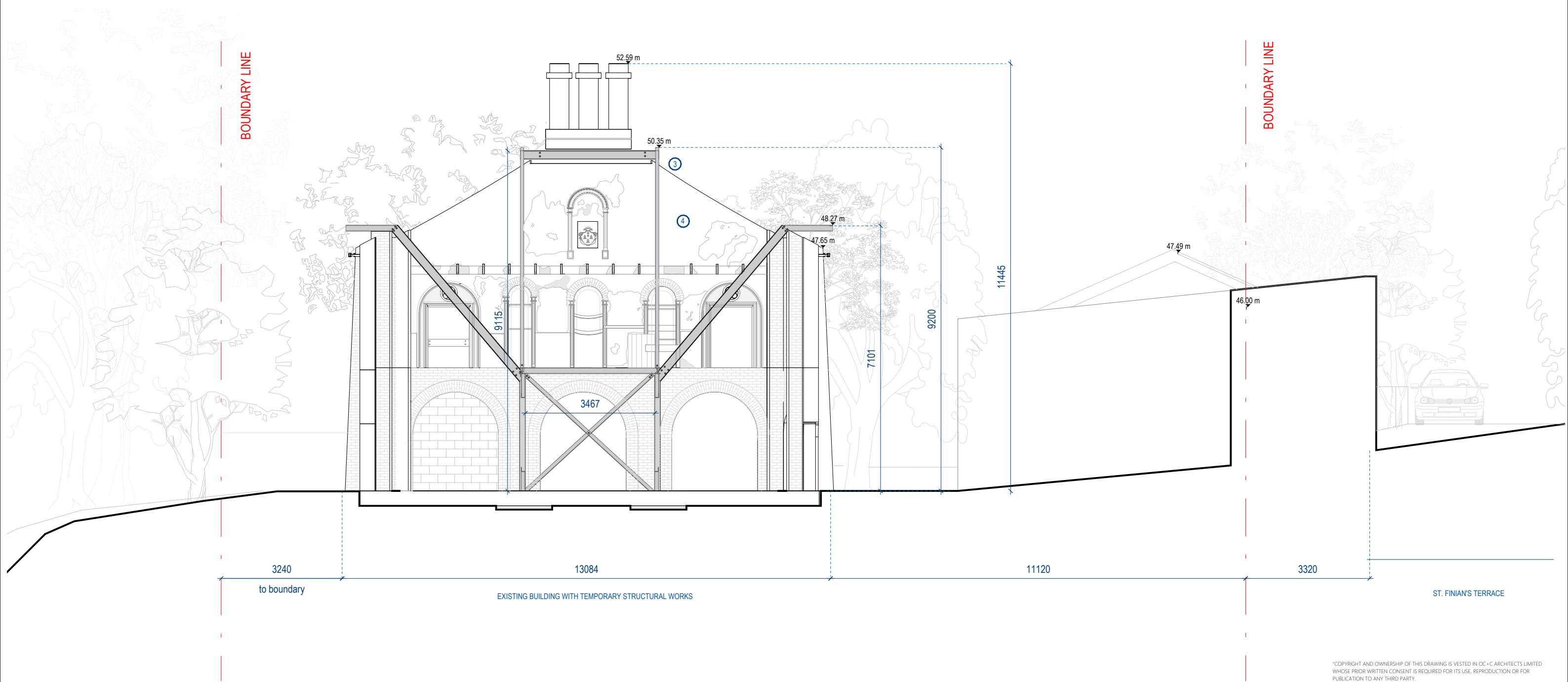
1 Section C-C (Existing) Scale - 1 : 100
