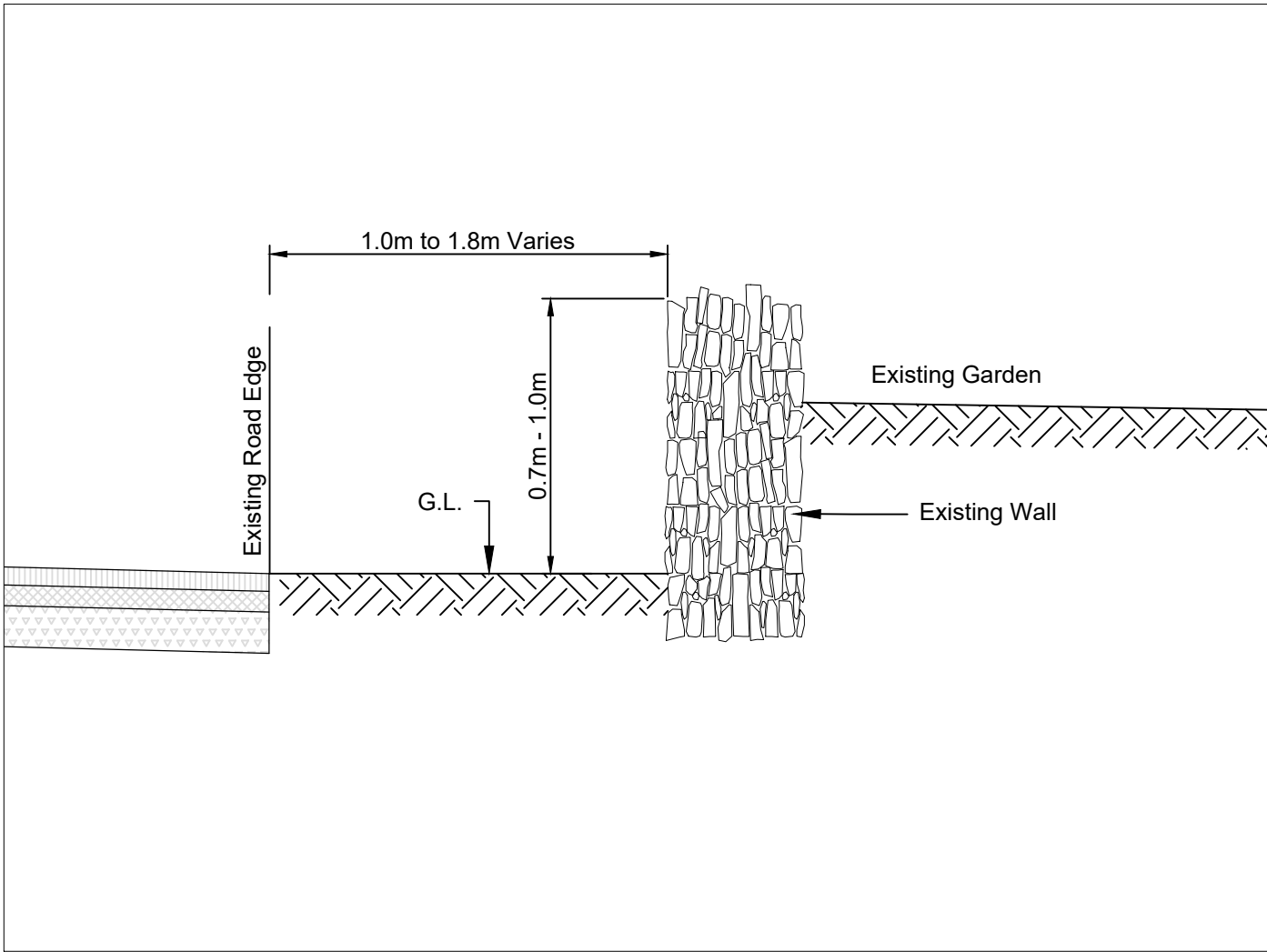
Section A - A Existing Wall Alignment 1:25
