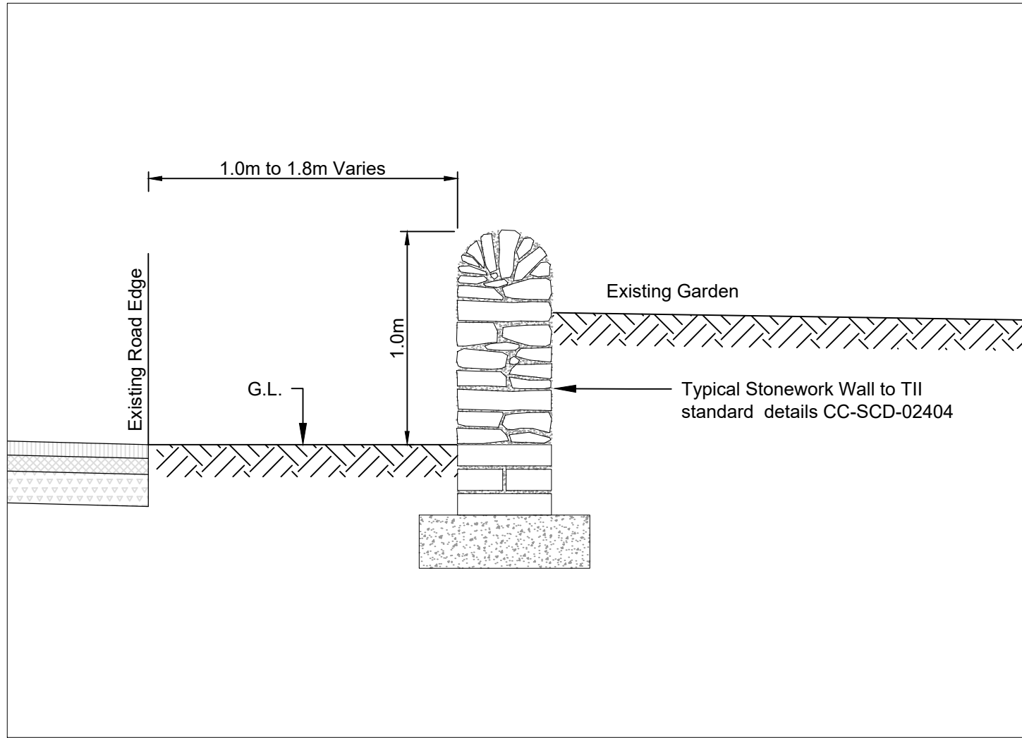
Section A - A Proposed Wall Alignment 1:25
