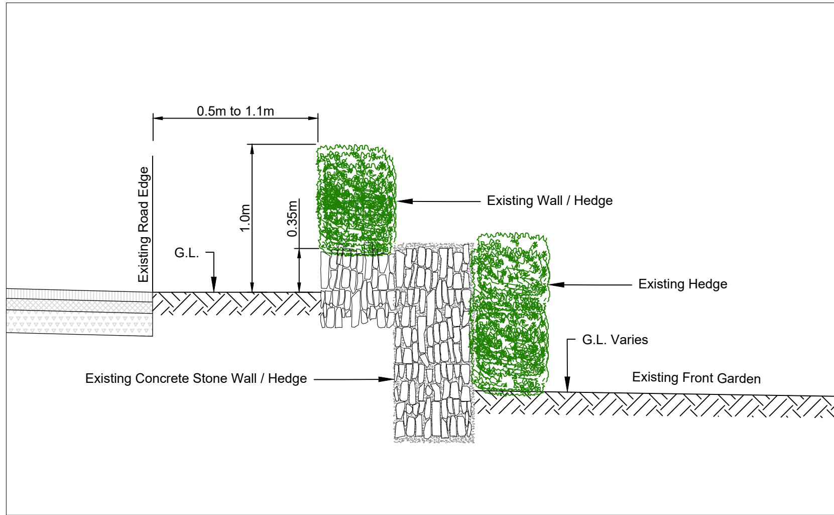
Section A - A Existing Wall Alignment 1:25
