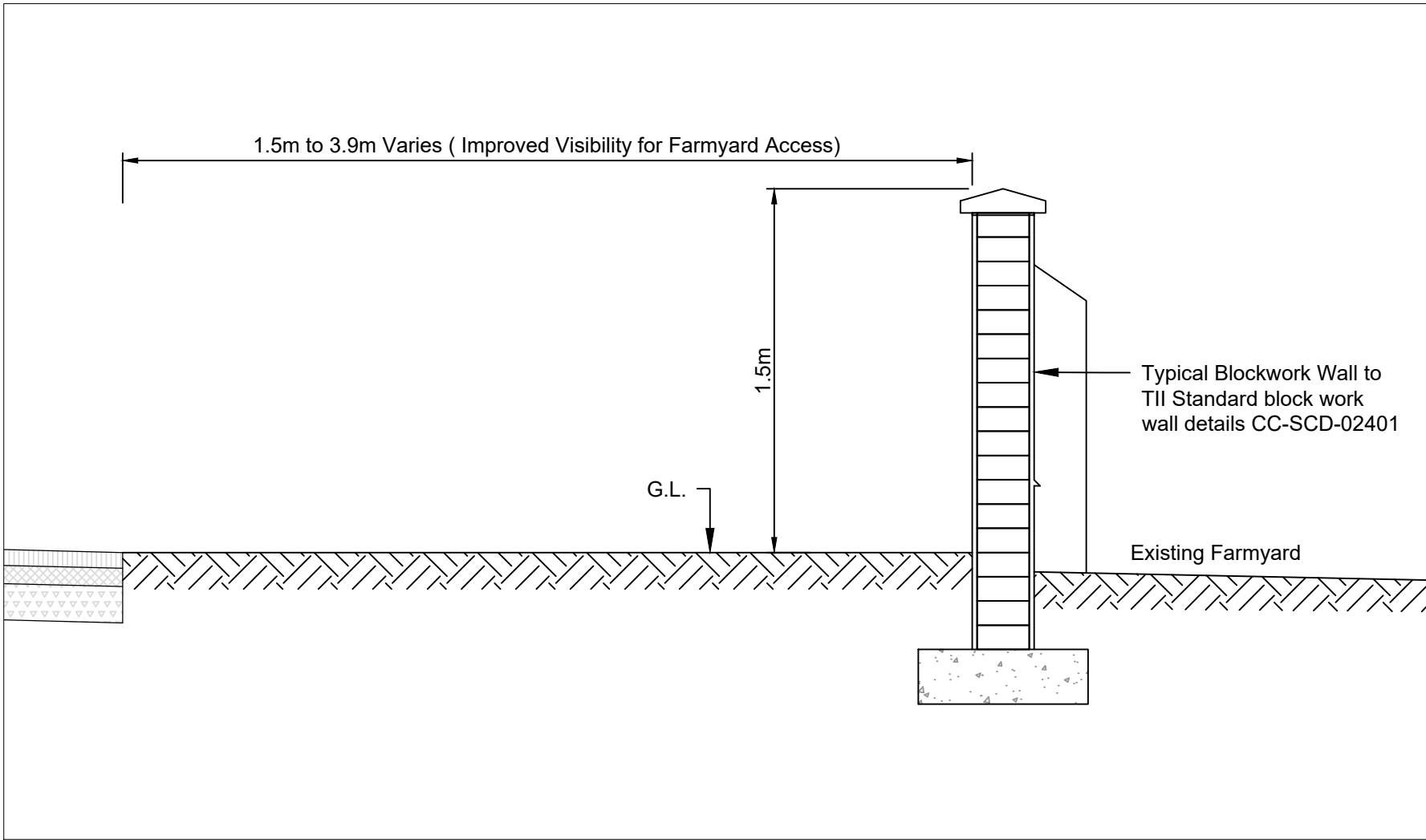
Section A - A Proposed Wall Alignment 1:25
