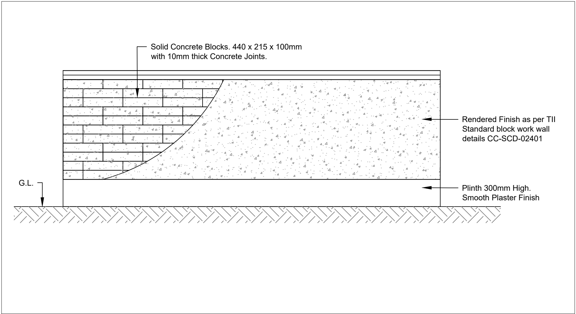
Typical Elevation Proposed Wall 1:25
