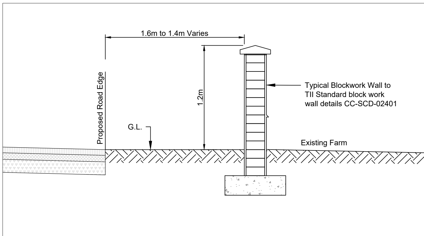
Section A - A Proposed Wall Alignment
