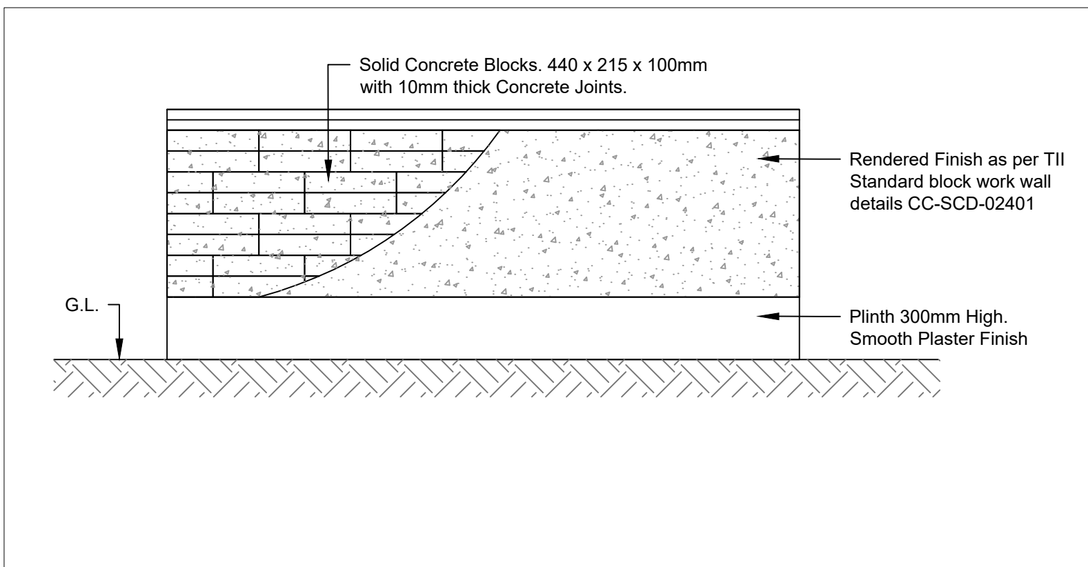
Proposed Wall Elevation
