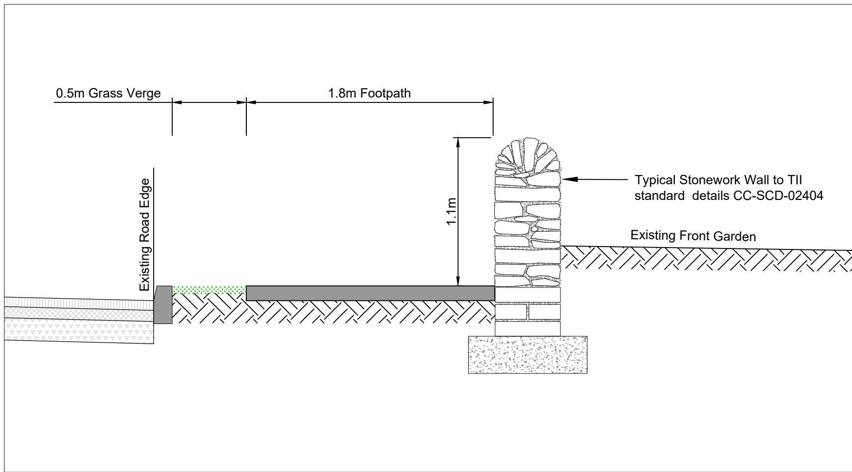
Section A - A Proposed Wall Alignment
