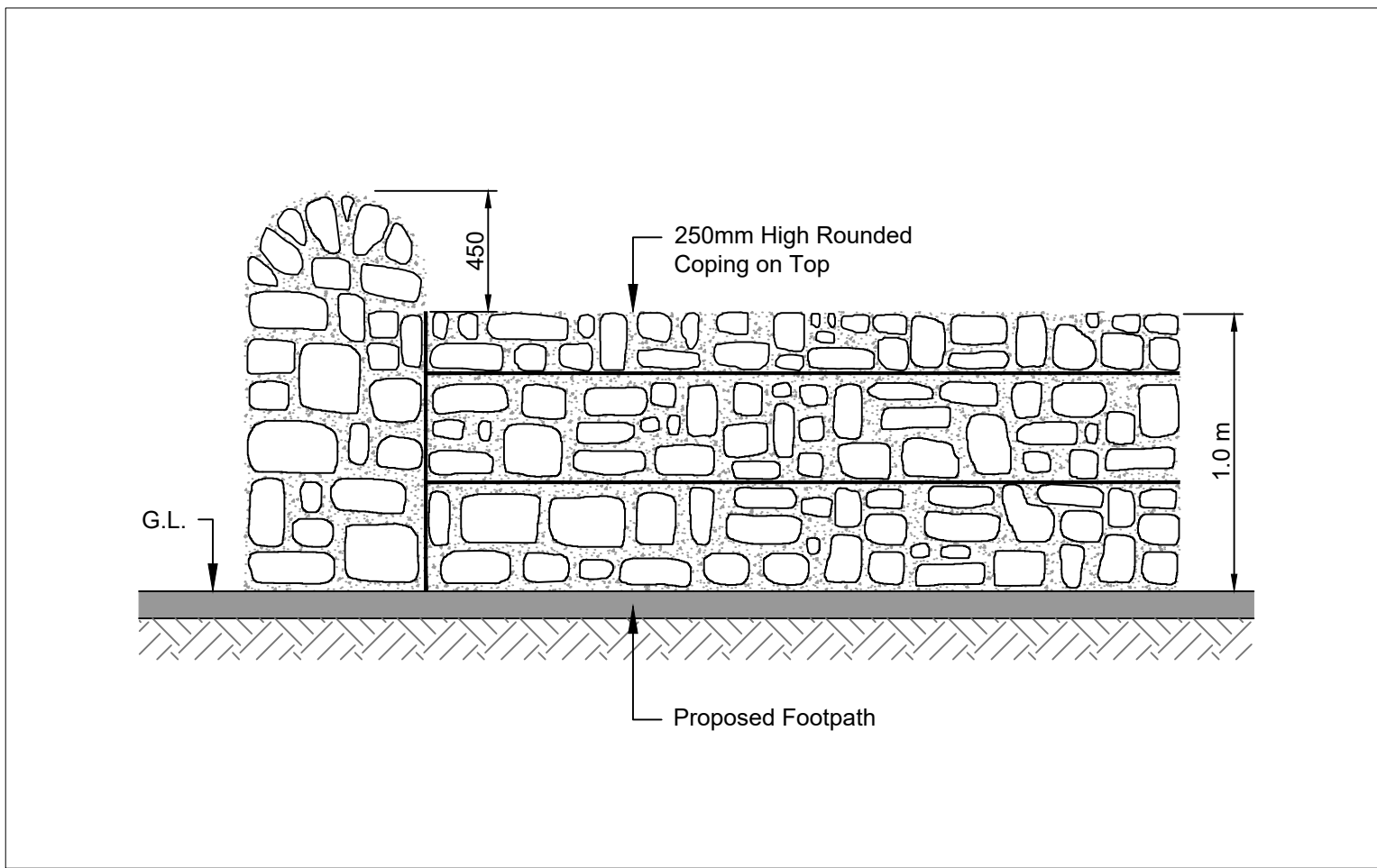
Typical Elevation Proposed Wall
