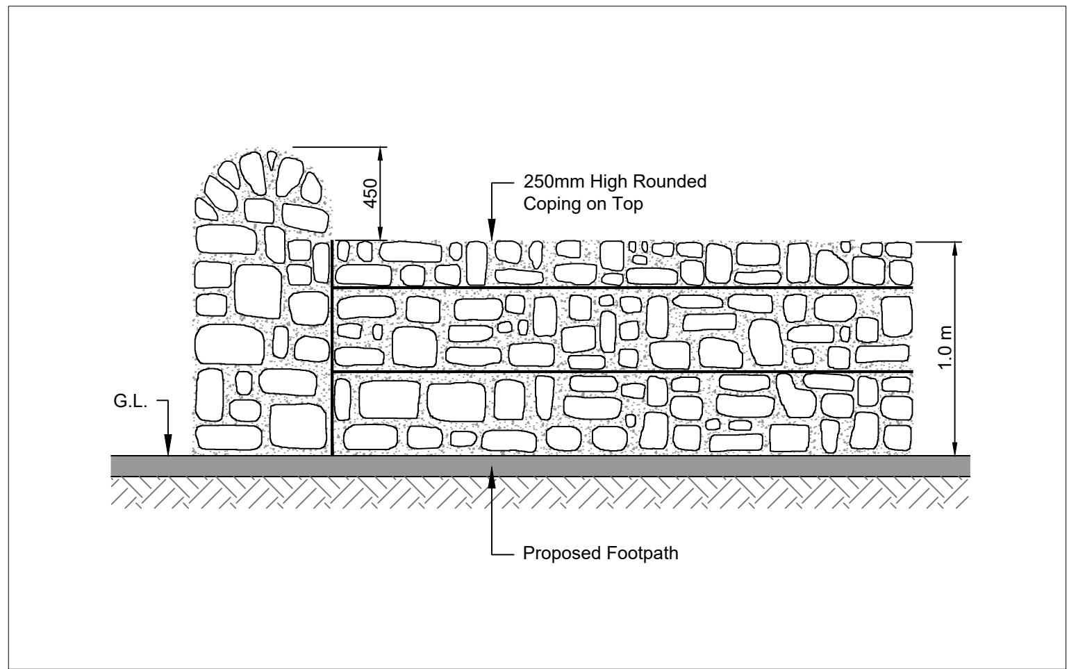
Typical Elevation Proposed Wall 1:25
