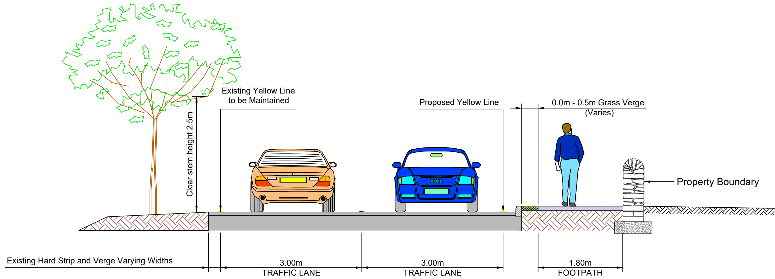
Typical Section (Looking West)
