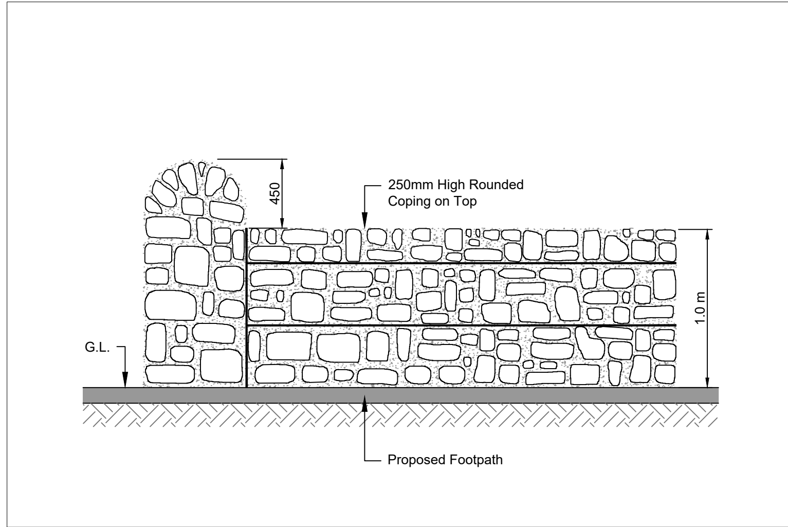
Typical Elevation Proposed Wall 1:25
