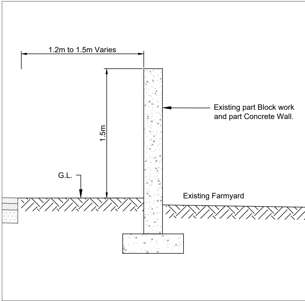
Section A - A Existing Wall Alignment 1:25
