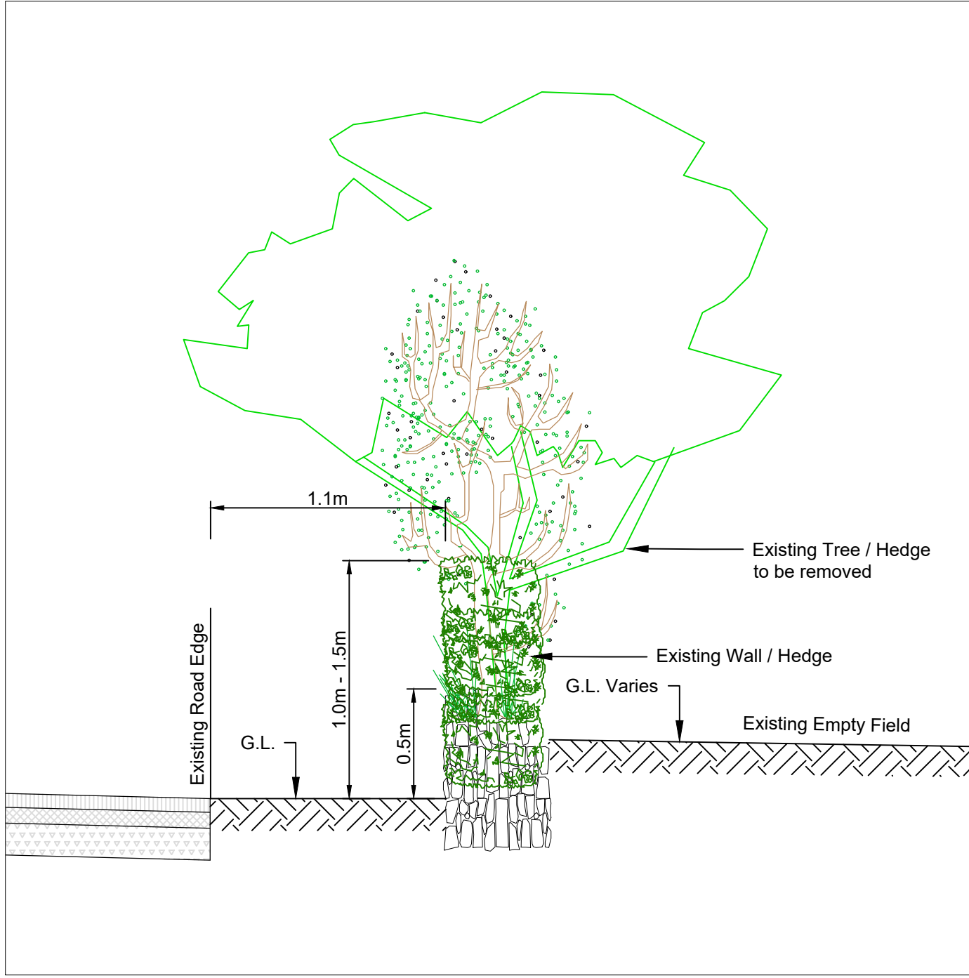
Section A - A Existing Wall Alignment 1:25
