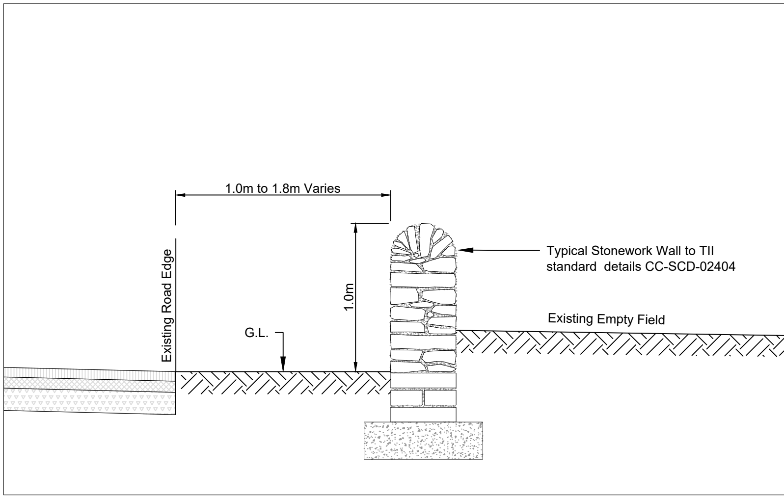
Section A - A Proposed Wall Alignment 1:25
