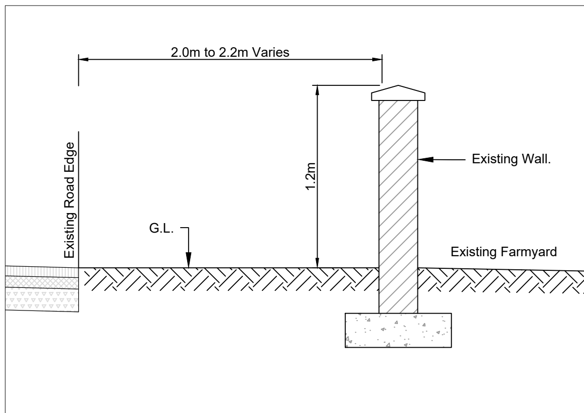
Section A - A Existing Wall Alignment
