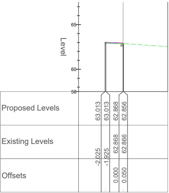
Chainage 70.000 (125)
