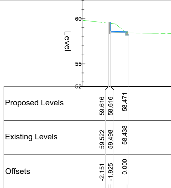
Chainage 210.000
