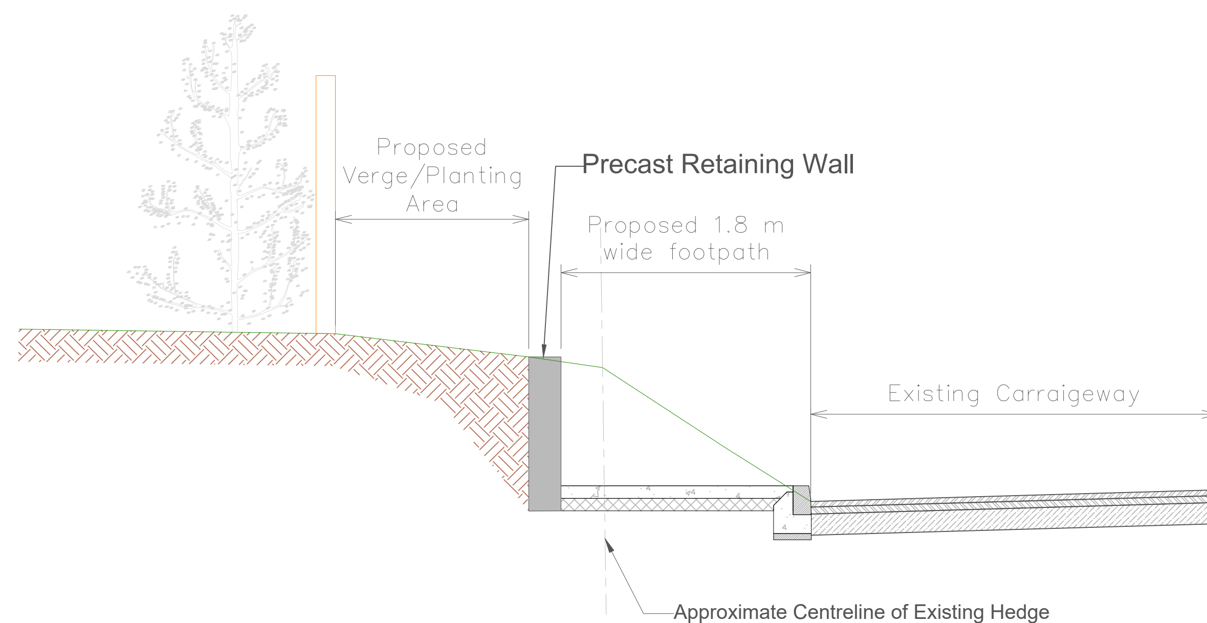
SECTION B-B Retaining Wall & Online Section Ch. 0+190-0+250
