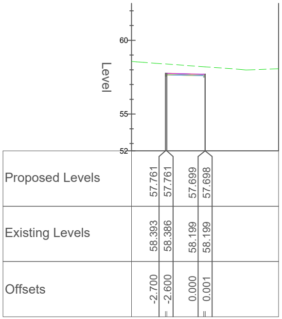
Chainage 180.000
