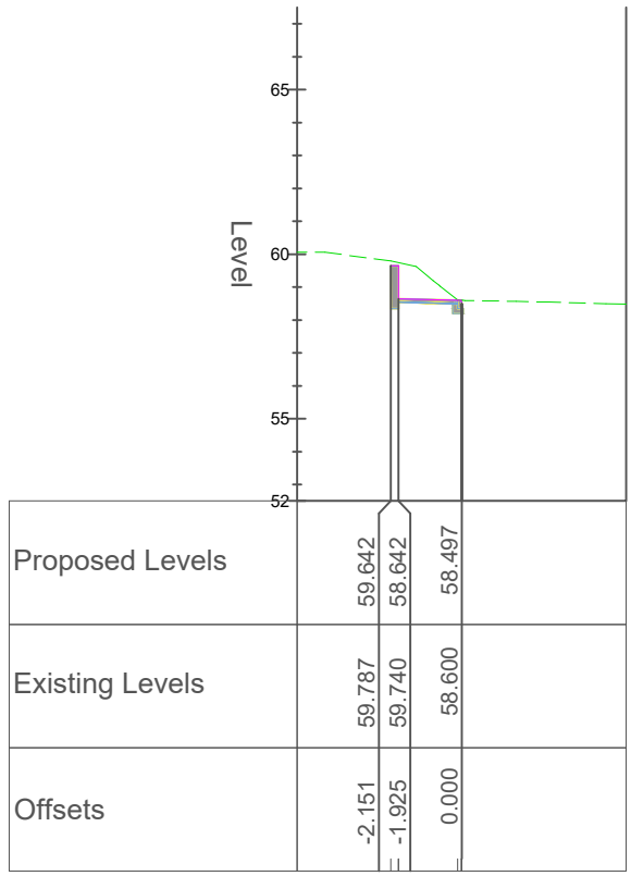
Chainage 210.000
