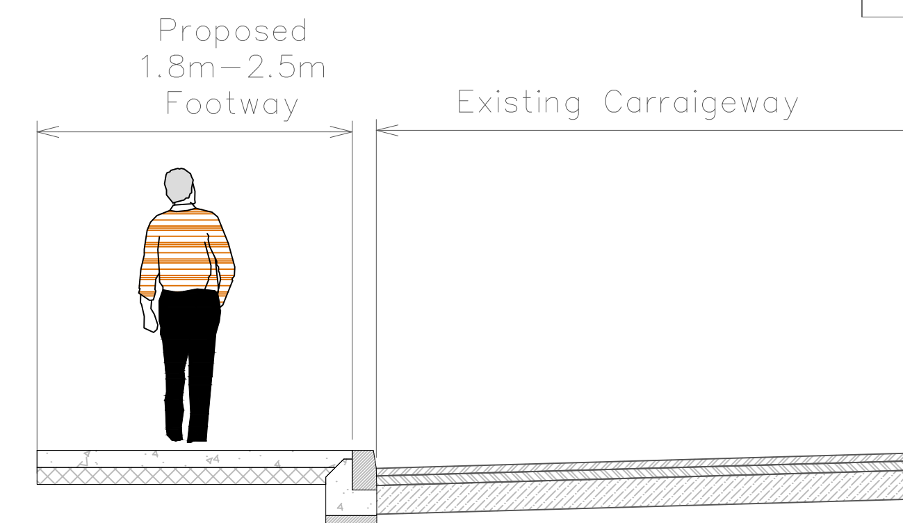
SECTION C-C Online Section Ch. 0+250-0+300
