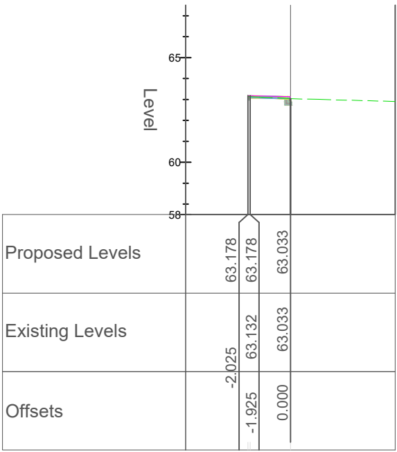
Chainage 50.000 (123)
