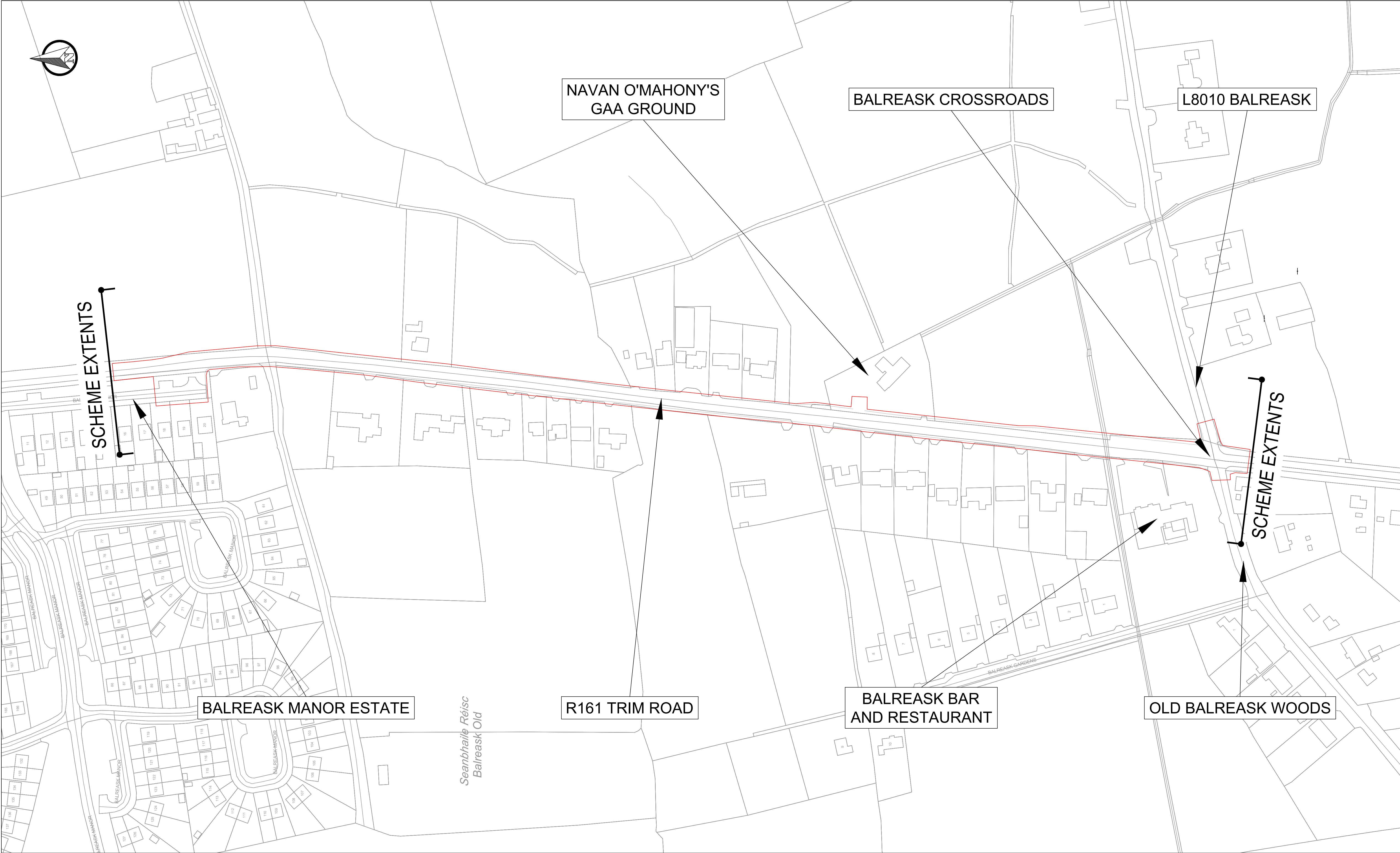
SITE LOCATION MAP 1:1250 @ A1 1:2500 @ A3
